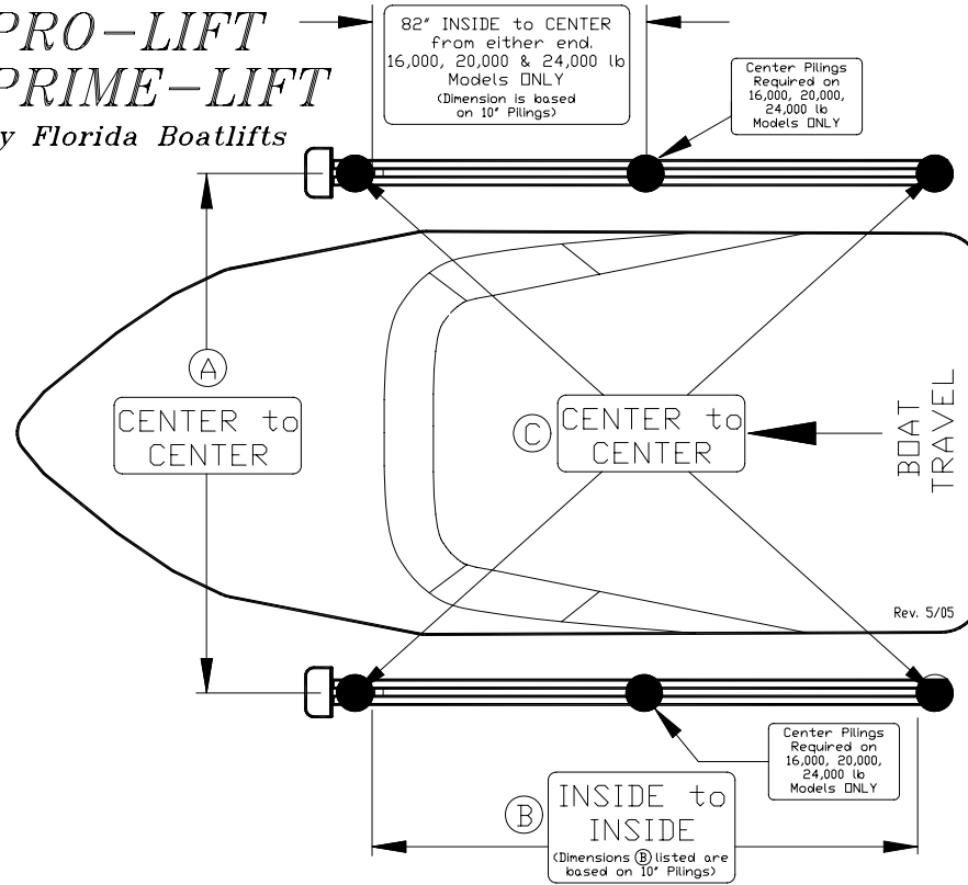
PILING PLACEMENT CHART
